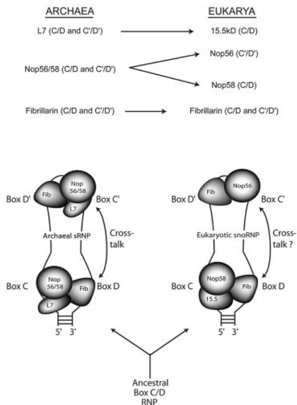
Fig. 7. Archaeal and eukaryotic box C/D RNP complexes exhibit symmetric versus asymmetric distribution of the RNP core proteins bound to sRNAs and snoRNAs, respectively. The illustrated structure of the eukaryotic snoRNP is based on the work of Cahill et al. (2002) and Szewczak et al. (2002).
