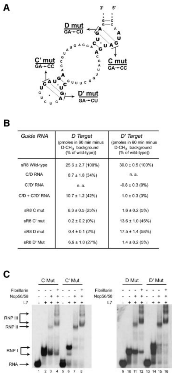
Fig. 4. Mutation of either the terminal box C/D core or internal C'/D' motifs in full-length sR8 affects guided 2'-O-methylation of both RNP complexes. (A) Schematic presentation of sR8 sRNA with various mutations in the box C, D, C' and D' sequences. For simplicity, the complete terminal helix is not shown but it is present in all mutant sRNAs. (B) Box C/D or C'/D' mutations affect methylation activity of both RNPs. Methylation efficiencies of wild-type sR8, halfmer RNAs and the full-length mutants are reported as total picomoles of methyl incorporation into the target RNAs in 1 h. Methylation of the control D-CH 3 or D'-CH 3 target is subtracted as background. Numbers in parentheses indicate the percentage of methylation with respect to activity of the respective RNPs in the full-length sR8 sRNA. (C) RNP complexes are assembled on sR8 box C/D and C'/D' RNA mutants. sR8 RNAs containing the individual mutants illustrated in (A) were radiolabeled and incubated with the sRNP core proteins as indicated above each gel lane. Assembled complexes were resolved on native polyacrylamide gels and visualized by autoradiography.
