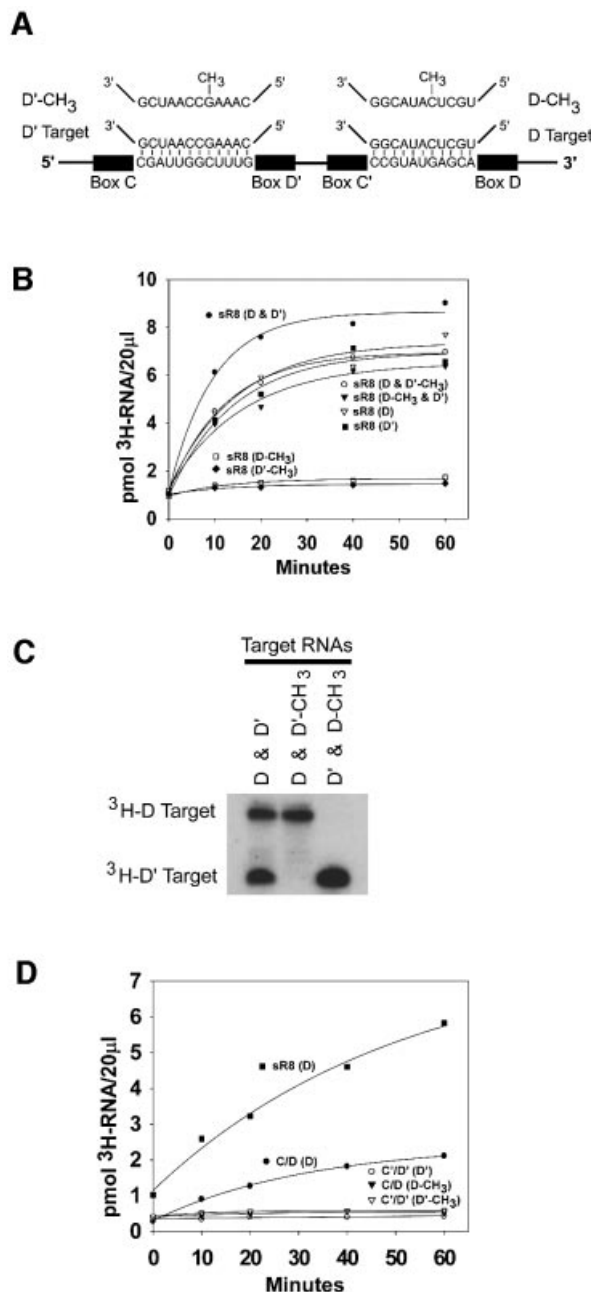
Fig. 3. In vitro assembled sR8 sRNP guides site-specific 2'-O-methylation from both terminal box C/D and internal C'/D' RNPs. Efficient methylation requires juxtapositioning of both RNP complexes in the full-length sRNA. (A) Schematic presentation of M. jannaschii sR8 base paired with D and D' target RNAs. D-CH 3 and D'-CH 3 target RNAs possessing a previously 2'-O-methylated sugar at the designate nucleotide are illustrated above. (B) The assembled sR8 sRNP complex guides site-specific methylation of both the D and D' target RNAs. Assembled sR8 sRNP was incubated at 70°C with the indicated target RNAs (in parentheses) and [ 3 H]SAM. At various times, aliquots of the reaction were collected and TCA precipitated, and [ 3 H]methyl incorporation was measured by scintillation counting. (C) Methylation of D and D' RNA substrates demonstrates site-specific 2'-O-methylation at designate nucleotides of the target RNAs. Target RNAs in various combinations indicated above the gel were resolved by electrophoresis and 2'-O-methylated RNAs revealed by radiography. (D) Efficient methylation requires juxtapositioned RNPs. RNP complexes assembled upon the box C/D and C'/D' halfmer RNAs were incubated with their respective target RNAs and assayed for methylation. sR8 (D) target RNA (solid square) is the control level of methylation for the box C/D core RNP when positioned in the full-length sR8 sRNP.
