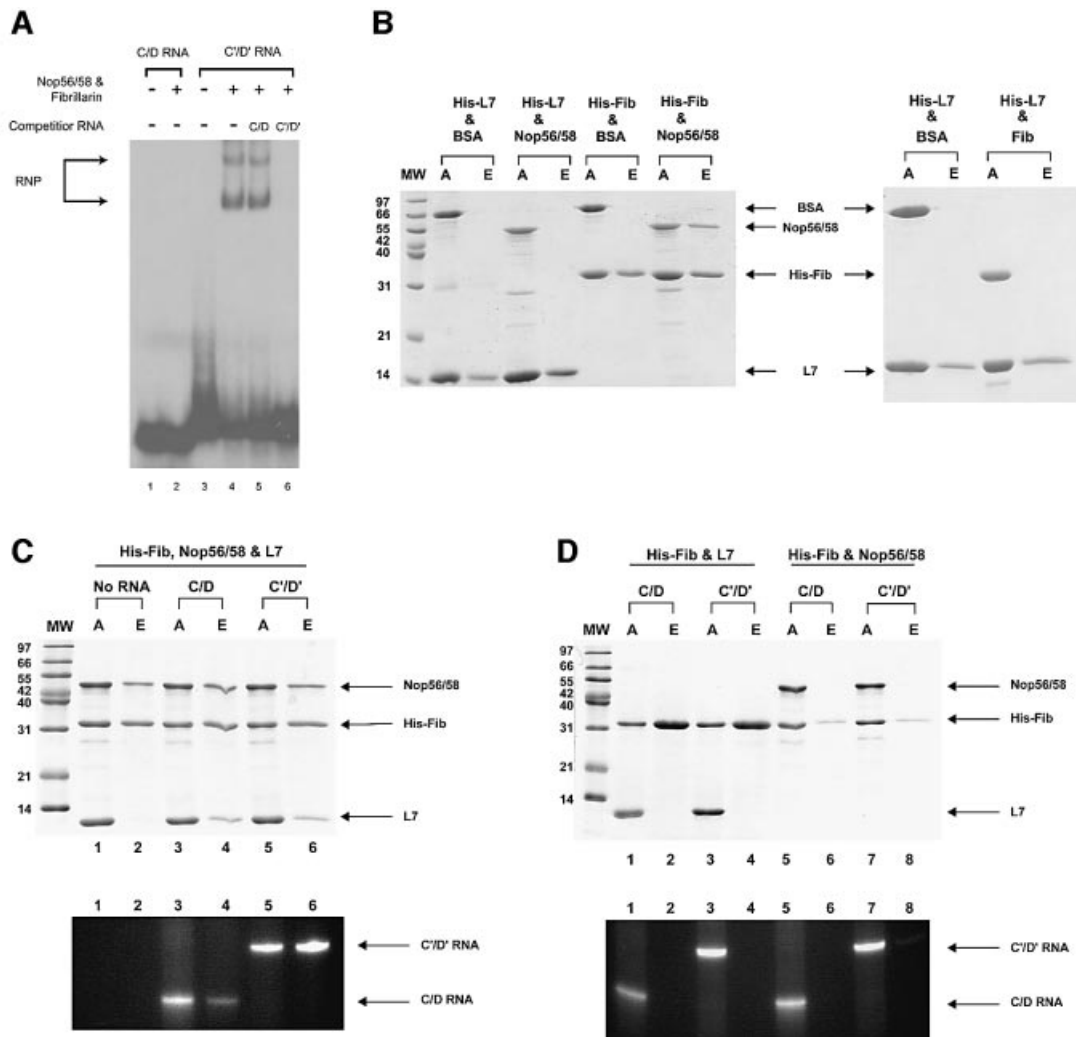
Fig. 2. Nop56/58 and fibrillar interact via protein-protein interactions and can bind the internal C'/D' motif in the absence of core protein L7. (A) Nop56/58 and fibrillar core proteins bind specifically to the C'/D' motif in the absence of L7 core protein. Nop56/58 and fibrillar were incubated with radiolabeled box C/D or C'/D' RNA. Assembled RNP complexes were resolved on a native polyacrylamide gel and visualized by autoradiography. Competition experiments included a 1000-fold molar excess of non-radiolabeled box C/D or C'/D' RNA. (B) Nop56/58 interacts with fibrillar. sRNP core proteins were incubated in equimolar concentrations. Twenty percent of the protein mixture was removed as the applied sample (A) and the remainder applied to affinity resin. Bound proteins were eluted (E), resolved on 14% SDS-polyacrylamide gels and visualized by Coomassie Blue staining. Incubated protein combinations are indicated above each gel lane. (C and D) Pull-down analysis demonstrates the presence of L7 in the C'/D' RNP complex. His-tagged fibrillar, Nop56/58 and L7 were incubated with the C/D and C'/D' RNAs in various combinations as indicated and fibrillar was affinity-selected via the His tag. Co-isolated sRNP core proteins (upper panels of C and D) and RNAs (lower panels of C and D) were resolved on polyacrylamide gels and visualized by Coomassie Blue and EtBr staining, respectively.
