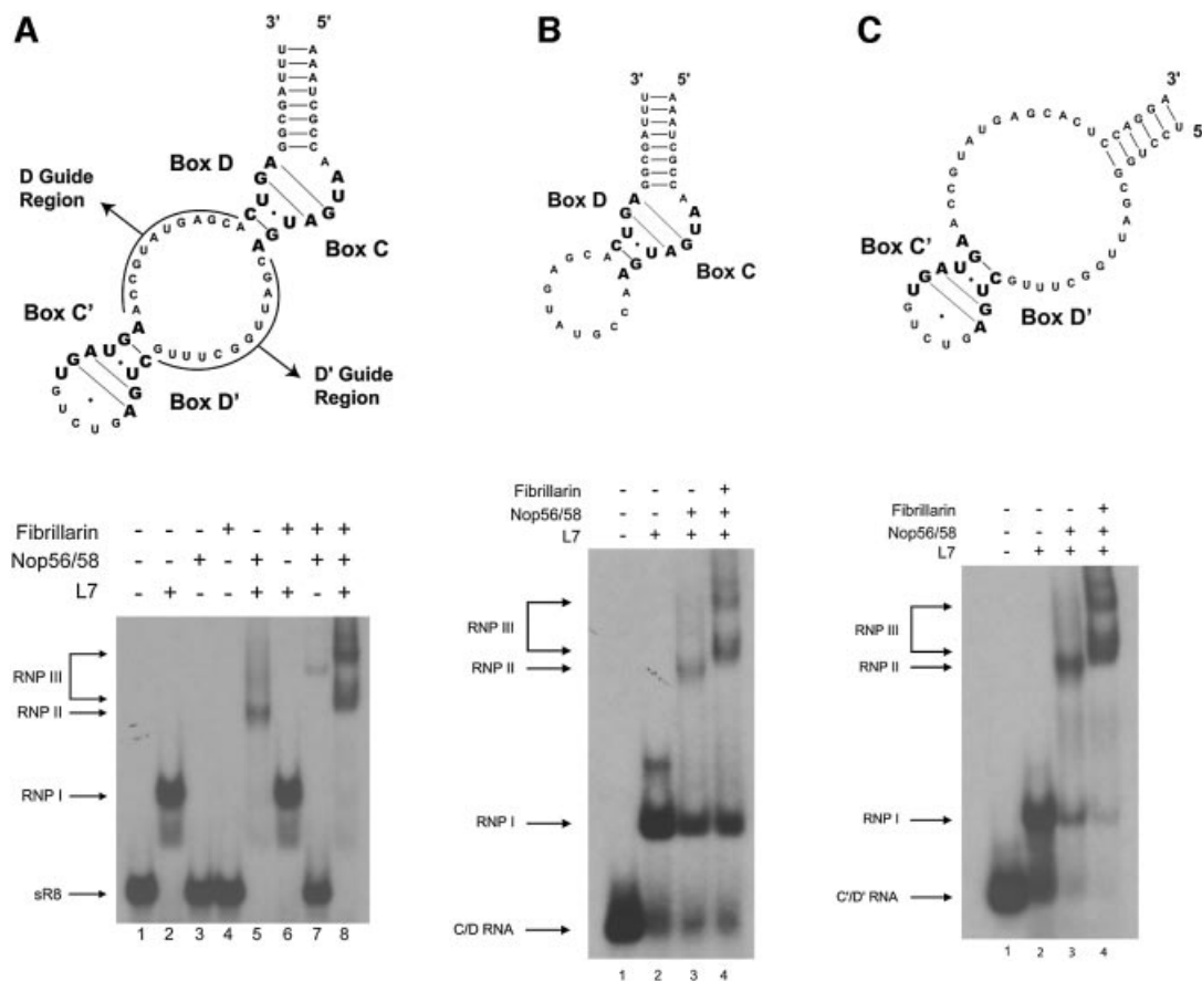
Fig. 1. Archaeal sR8 sRNP assembly requires a defined order of core protein addition and forms symmetric RNP complexes on the terminal box C/D core and internal C'/D' motifs. (A) The folded structure of M. jannaschii sR8 sRNA with terminal box C/D core and internal C'/D' motifs is based upon the consensus structure of the snoRNA box C/D motif implied from the crystal structure of the 15.5 kDa binding site on the U4 snRNA (Vidovic et al. , 2000; Watkins et al. , 2000). Lower panel: sR8 sRNP complexes were assembled by incubating L7, Nop56/58 and fibrillarin core proteins, either individually or in different combinations, with 5'-radiolabeled sR8 sRNA. Assembled complexes were resolved on 4% native polyacrylamide gels and RNPs were visualized by autoradiography. Migration positions of the partially assembled (RNP I and RNP II) and complete (RNP III) RNP complexes are indicated. (B and C) The terminal box C/D core and internal C'/D' RNA half-molecules are derived from the wild-type sR8 full-length sRNA. Lower panels: terminal box C/D core and internal C'/D' RNPs were assembled by incubating 5'-radiolabeled RNA with the indicated sRNP core proteins. Migration positions of the partial (RNP I and RNP II) and fully assembled RNPs (RNP III) are indicated. The slower migrating complex in lane 2 of (C) is non-specific L7 binding to the RNA at elevated L7 concentrations.
