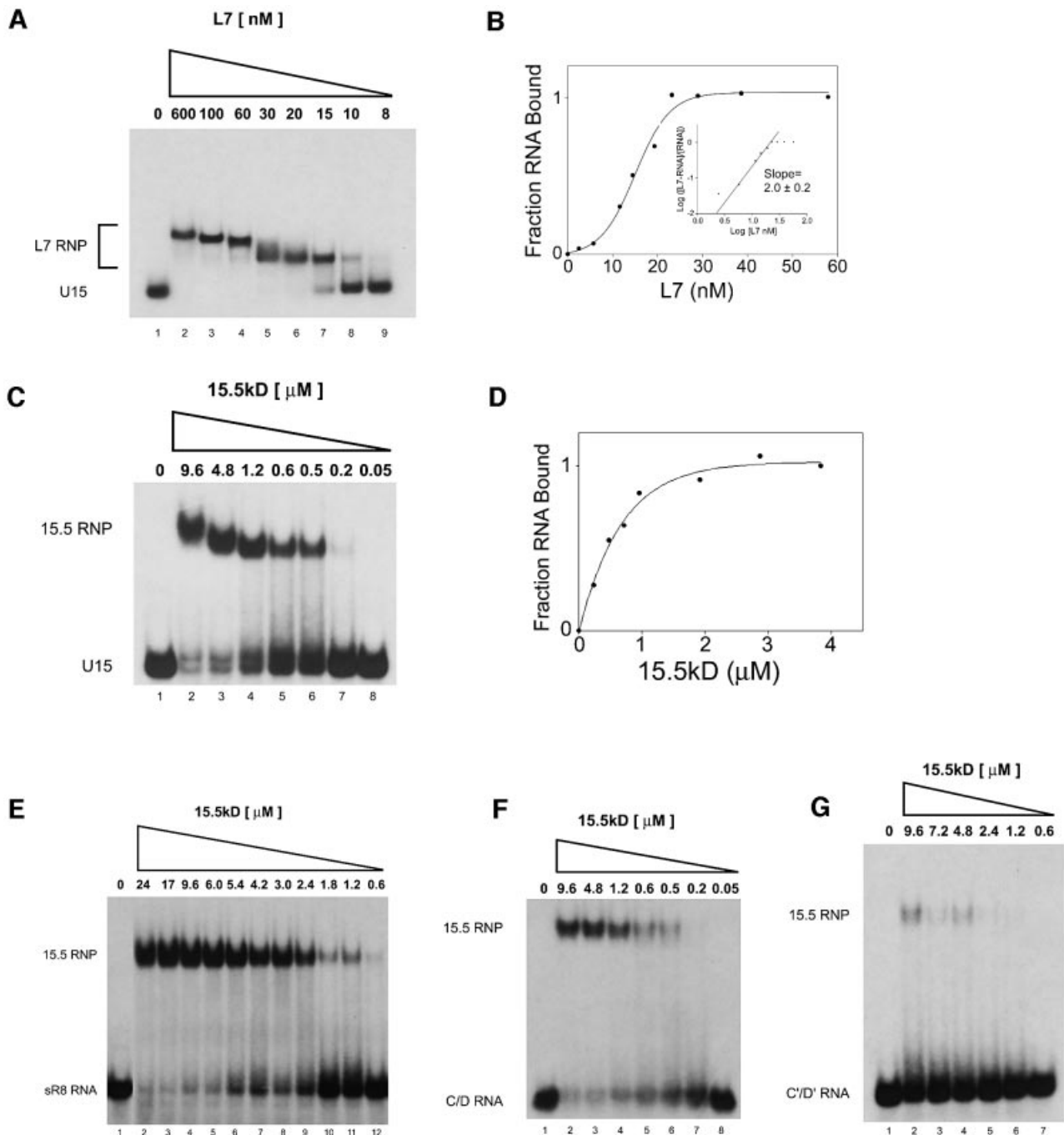
Fig. 6. Archaeal L7 binds both the C/D and C'/D' motifs, while eukaryotic 15.5 kDa protein binds only the terminal box C/D core motif. (A) Increasing amounts of M.jannaschii L7 protein were incubated with radiolabeled human U15 snoRNA. Assembled RNP complexes were resolved on a native polyacrylamide gel and visualized by autoradiography. (B) Archaeal sRNP core protein L7 exhibits cooperativity in binding to U15 snoRNA. Binding analyses were performed as detailed in Figure 5. (C) Eukaryotic snoRNP core protein 15.5 kDa binds only the U15 box C/D core motif. Increasing amounts of mouse 15.5 kDa protein were incubated with radiolabeled human U15 snoRNA. Assembled RNP complexes were resolved on a native polyacrylamide gel and visualized by radiography. (D) The fraction of U15 snoRNA bound in an RNP complex is plotted as a function of 15.5 kDa concentration. Increasing amounts of mouse 15.5 kDa core protein were incubated with radiolabeled full-length archaeal sR8 sRNA (E) and halfmer RNAs possessing either the terminal box C/D (F) or internal C'/D' (G) motifs. Assembled RNP complexes were resolved on native polyacrylamide gels and visualized by radiography.
